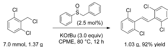
Scheme 3. Formation of 2,2',6,6'-tetrachlorostilbene on gram scale.
