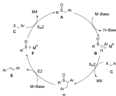
Scheme 2. Proposed mechanism of the sulfenate-anion-catalyzed coupling of benzyl halides to form symmetric stilbenes.
